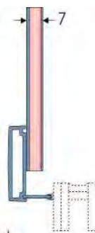
Tipo KV 7 Up 3.1 W/m 2 k Kg 5,0 m 2
