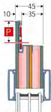
Tipo EV 45 Up 0.65 W/m²k Rw 33 dB Kg 21,0 m²
