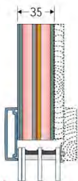
Tipo TM 35 Up 0.86 W/m²k Rw 33 dB Kg 18,0 m²
